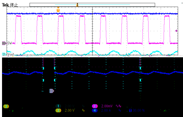
Figure 19. Output Ripple ( I_{LOAD}=3A )
