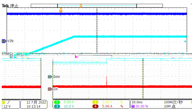
Figure 14. Enable Threshold
