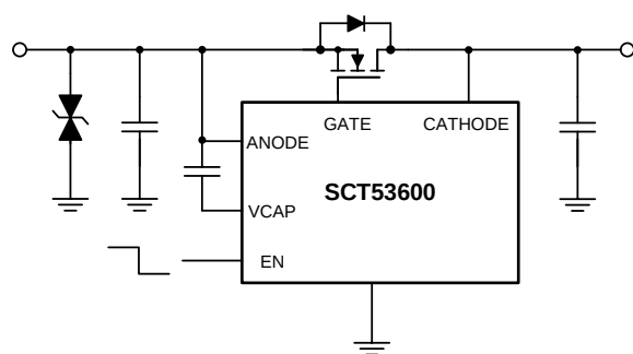
Typical Application
