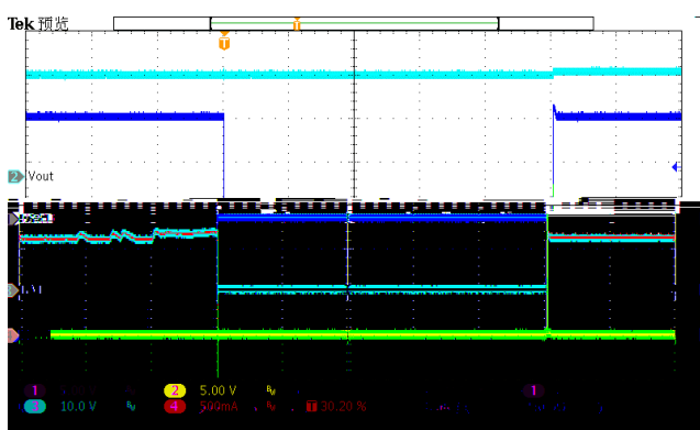
Figure 19. Input Micro-Short
