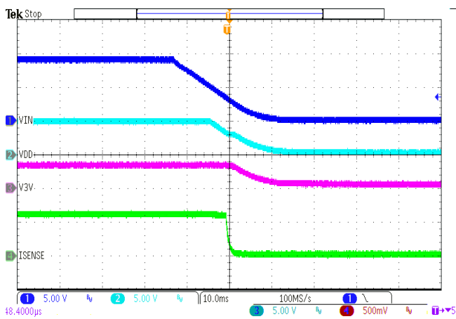
Figure 14. Power Down
