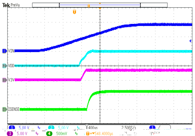
Figure 12. Power Up
