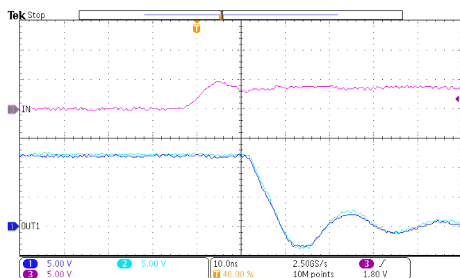
Figure 16. Driver INA-/INB- Switching OFF
