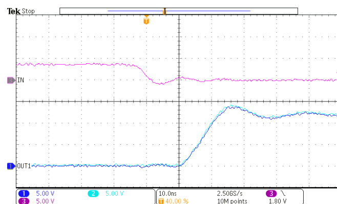
Figure 17. Driver INA-/INB- Switching ON
