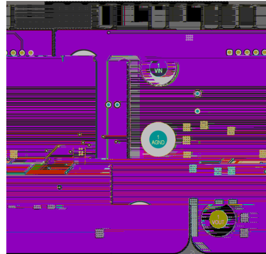
Figure 5. Internal 1 Layer
