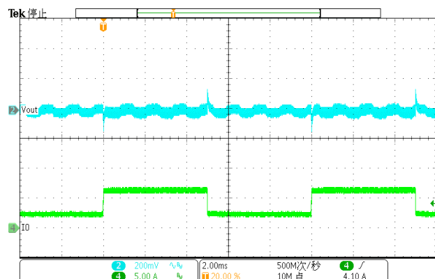
Figure 12. Load Transient (2A-6A, SR=1600mA/us, CH-1: Iout, CH-2: Vout)
