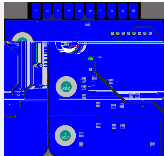
Figure 7. Bottom Layer
